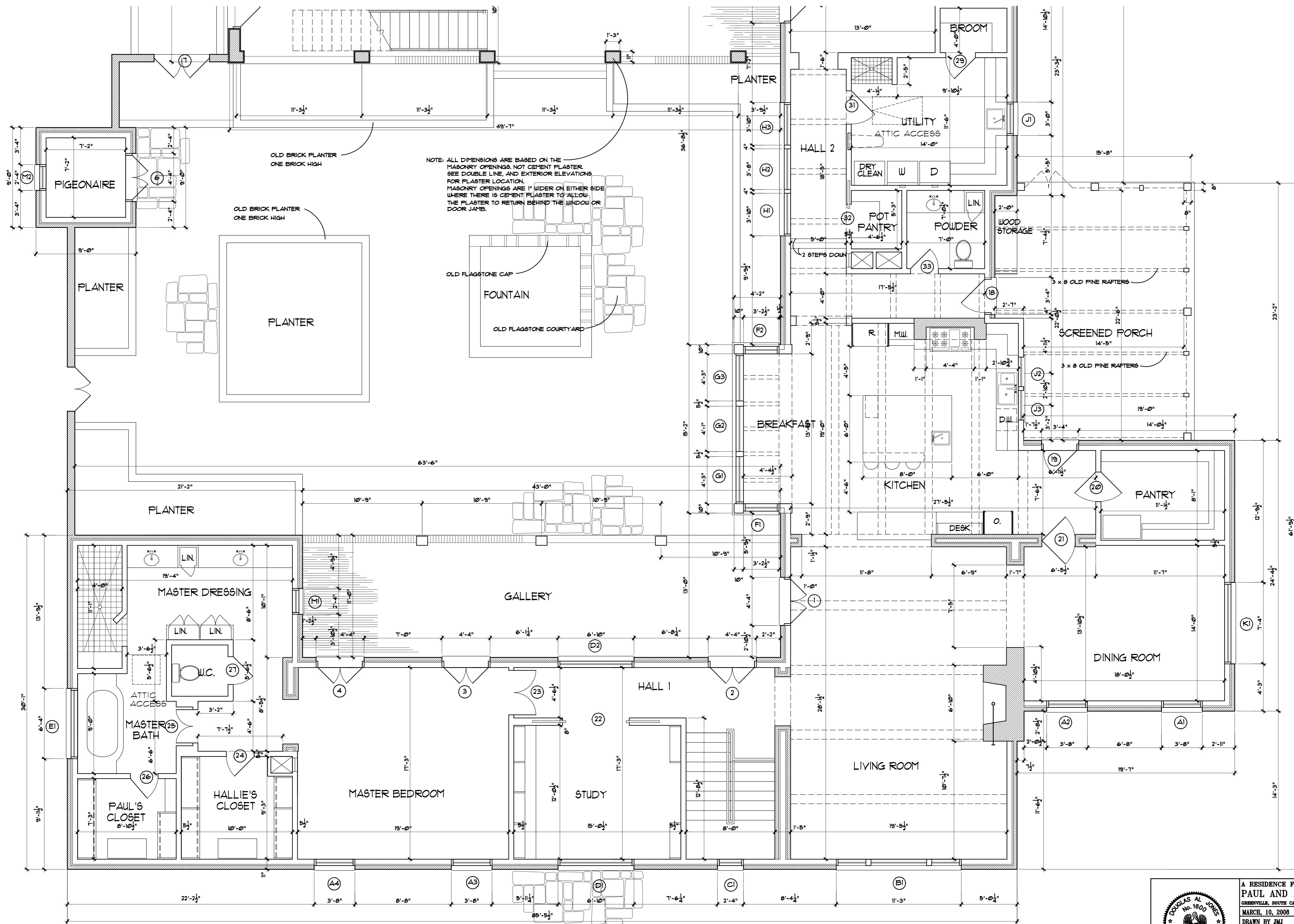
1 PARTIAL FIRST FLOOR PLAN SCALE: 1/4" = 1'-0"
