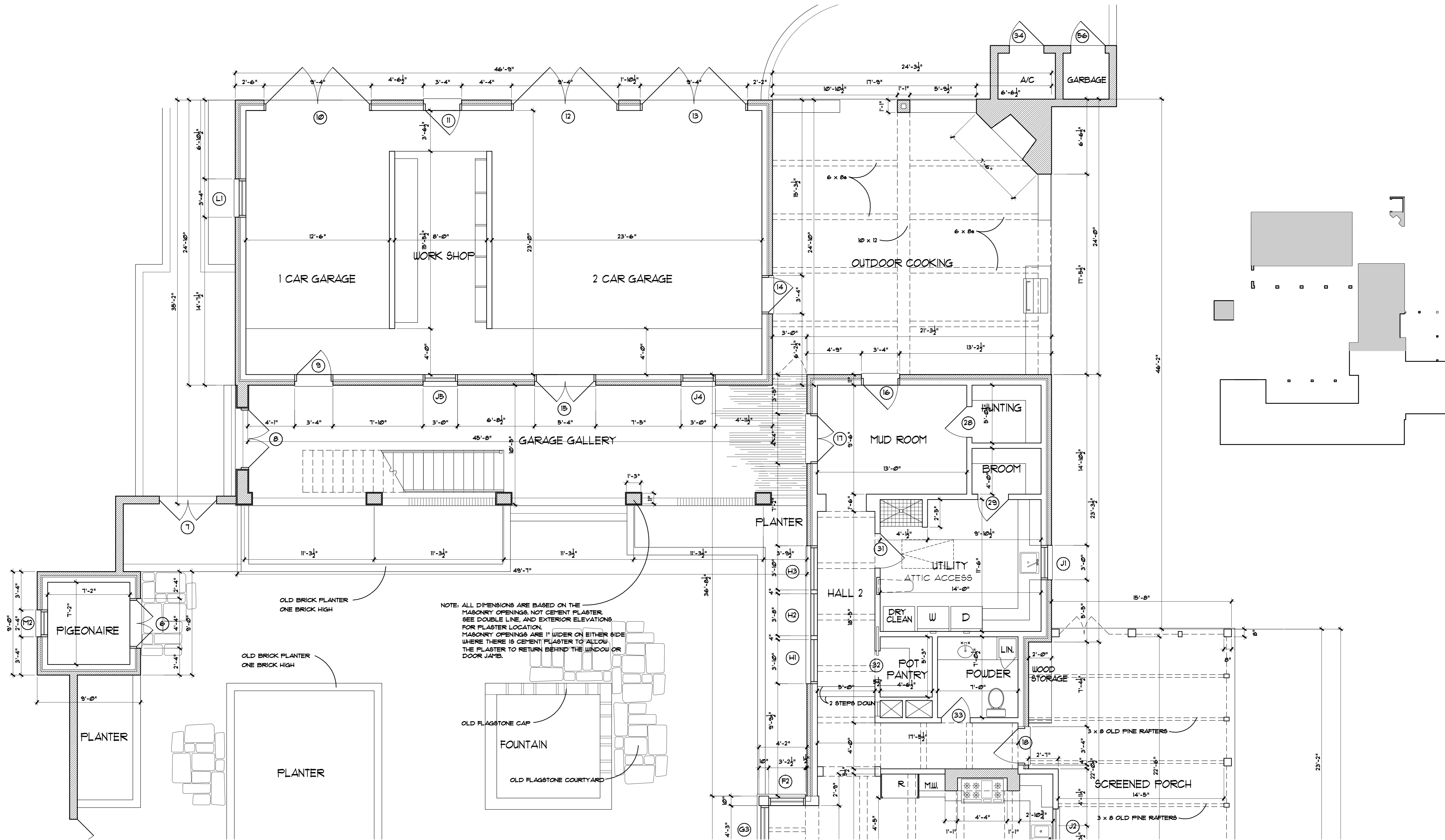
1 PARTIAL FIRST FLOOR PLAN SCALE: 1/4" = 1'-0"
